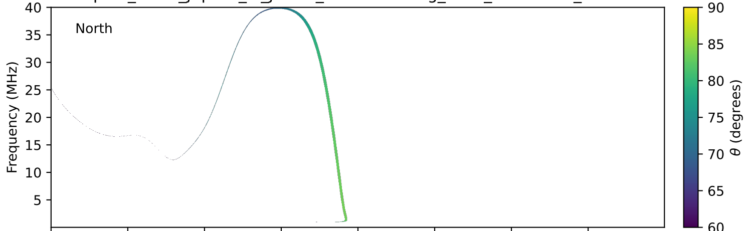
expres_earth_jupiter_io_jrm33_lossc-wid1deg_3kev_20150225_v11.cdf
