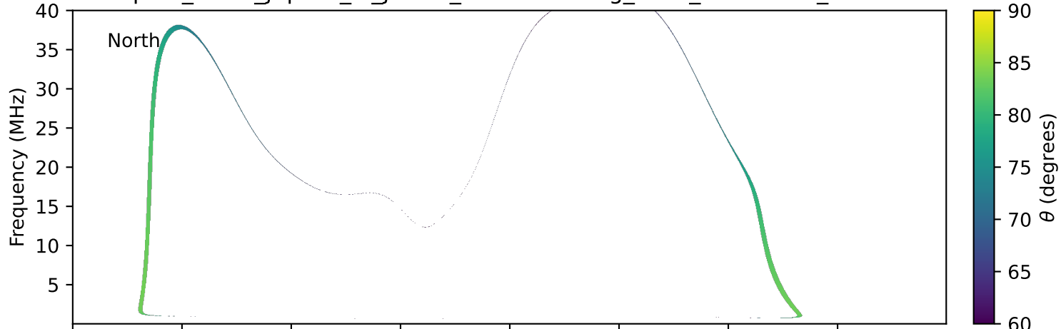
expres_earth_jupiter_io_jrm33_lossc-wid1deg_3kev_20150214_v11.cdf
