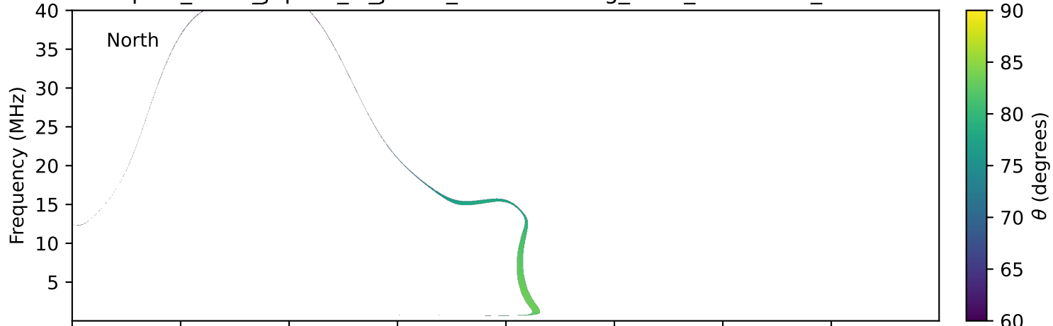
expres_earth_jupiter_io_jrm33_lossc-wid1deg_3kev_20150209_v11.cdf
