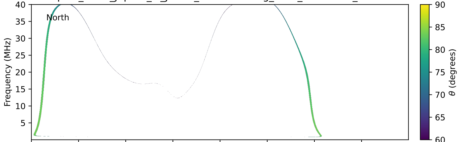
expres_earth_jupiter_io_jrm33_lossc-wid1deg_3kev_20150207_v11.cdf
