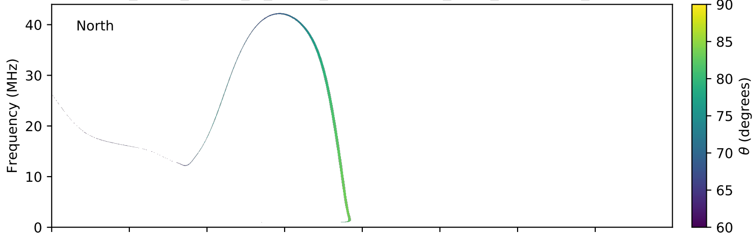
expres_earth_jupiter_io_jrm09_lossc-wid1deg_3kev_20150225_v01.cdf
