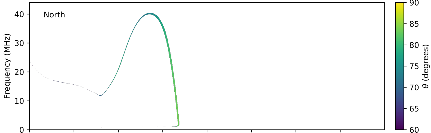
expres_earth_jupiter_io_jrm09_lossc-wid1deg_3kev_20150218_v01.cdf
