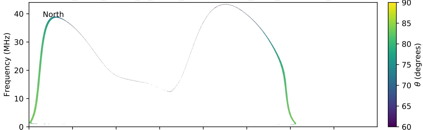
expres_earth_jupiter_io_jrm09_lossc-wid1deg_3kev_20150207_v01.cdf
