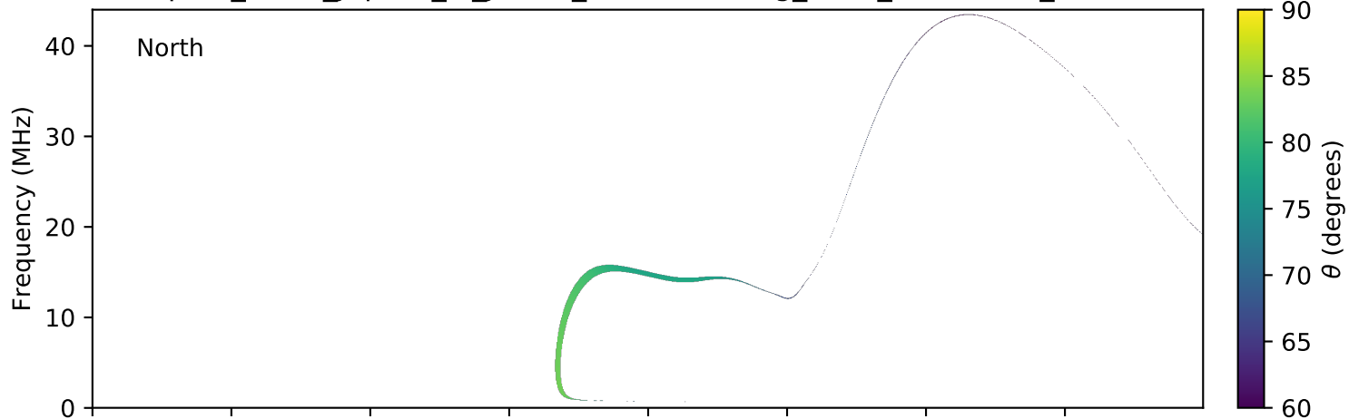
expres_earth_jupiter_io_jrm09_lossc-wid1deg_3kev_20150203_v01.cdf
