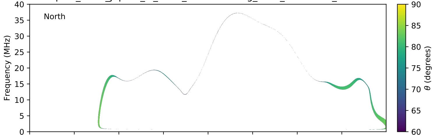
expres_earth_jupiter_io_isaac_lossc-wid1deg_3kev_20150228_v01.cdf
