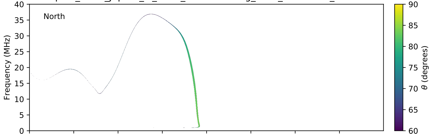
expres_earth_jupiter_io_isaac_lossc-wid1deg_3kev_20150225_v01.cdf
