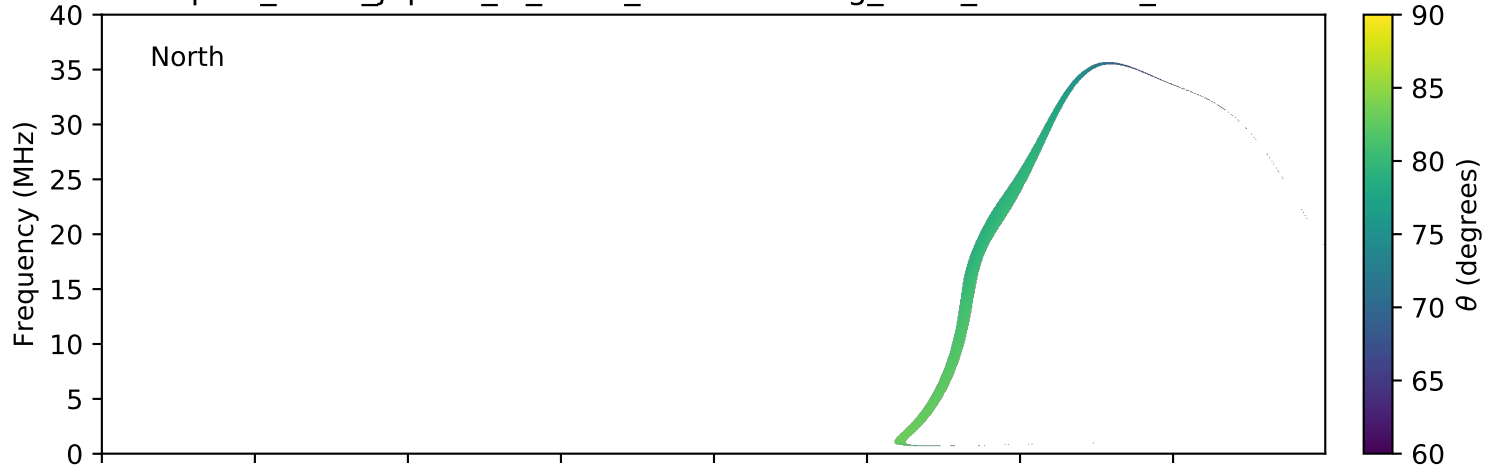
expres_earth_jupiter_io_isaac_lossc-wid1deg_3kev_20150224_v01.cdf
