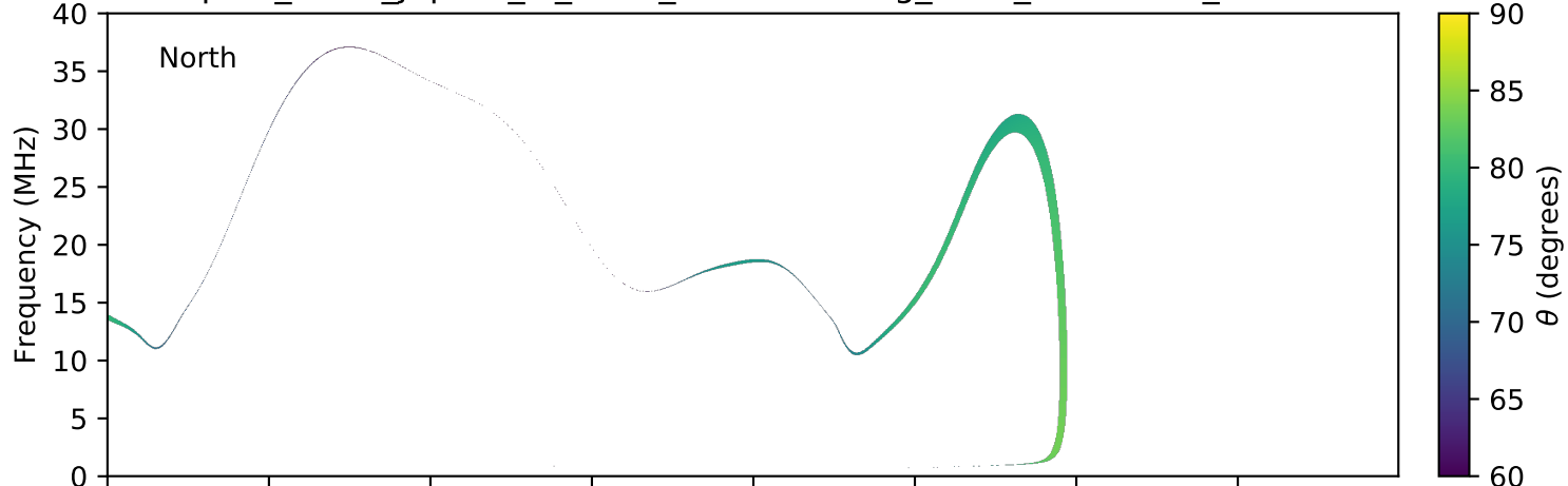
expres_earth_jupiter_io_isaac_lossc-wid1deg_3kev_20150223_v01.cdf
