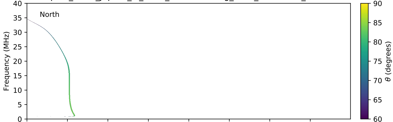
expres_earth_jupiter_io_isaac_lossc-wid1deg_3kev_20150220_v01.cdf
