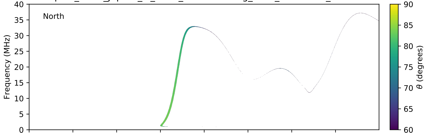
expres_earth_jupiter_io_isaac_lossc-wid1deg_3kev_20150219_v01.cdf
