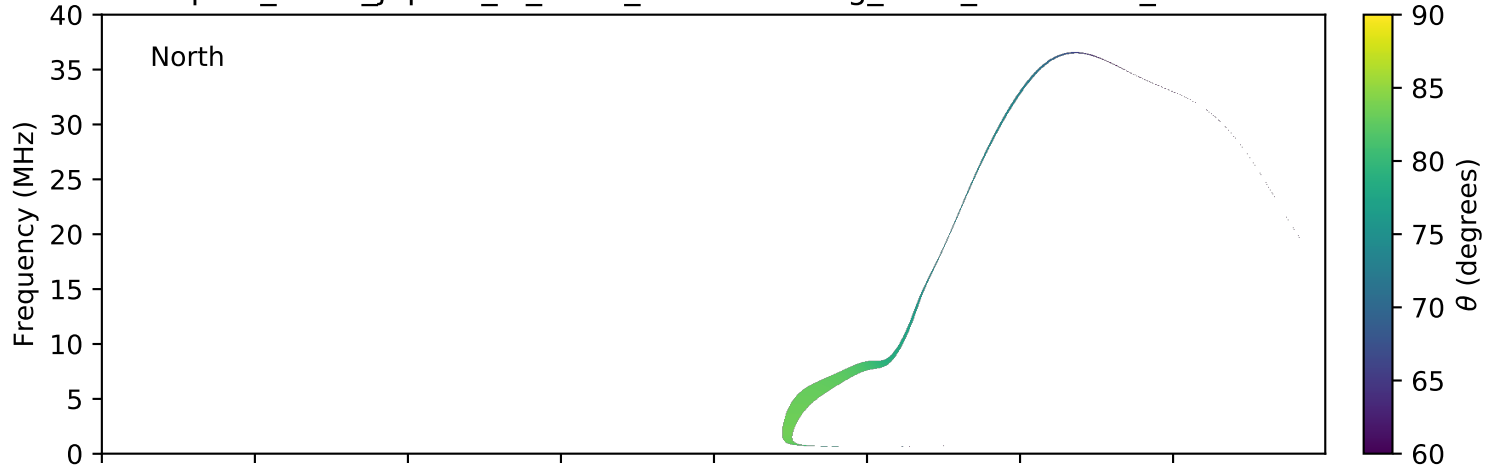
expres_earth_jupiter_io_isaac_lossc-wid1deg_3kev_20150217_v01.cdf
