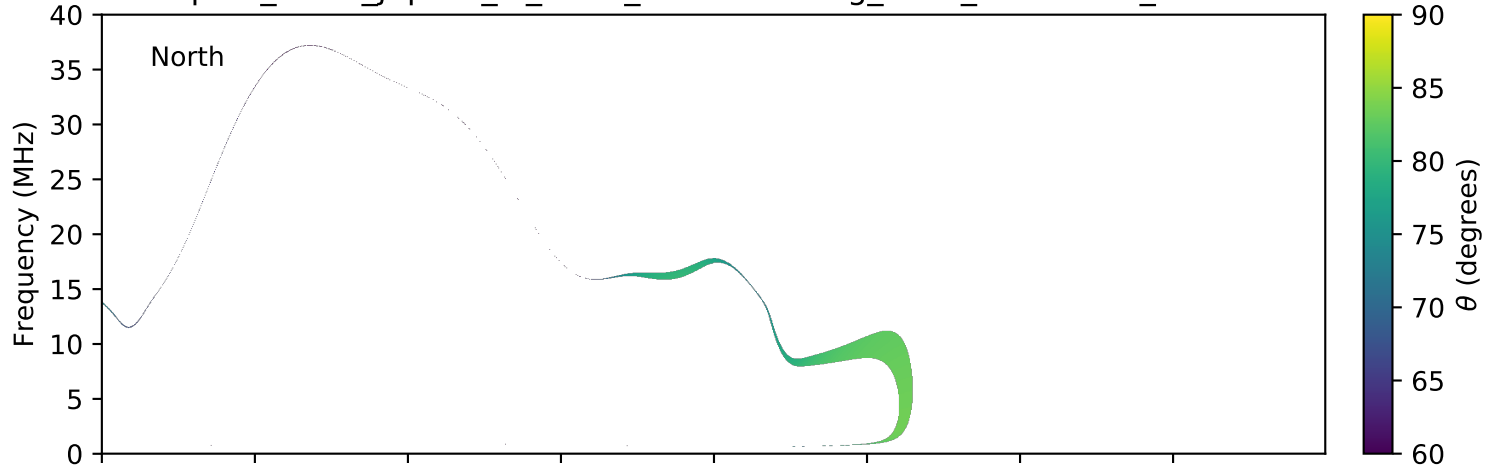
expres_earth_jupiter_io_isaac_lossc-wid1deg_3kev_20150216_v01.cdf
