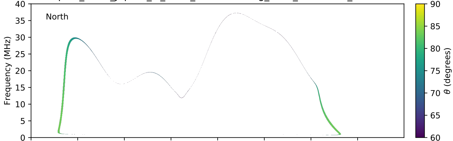
expres_earth_jupiter_io_isaac_lossc-wid1deg_3kev_20150214_v01.cdf
