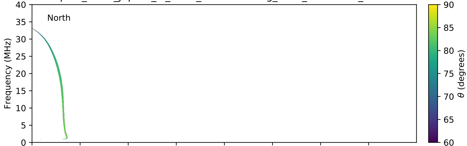
expres_earth_jupiter_io_isaac_lossc-wid1deg_3kev_20150213_v01.cdf
