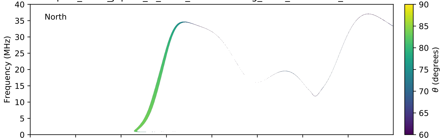
expres_earth_jupiter_io_isaac_lossc-wid1deg_3kev_20150212_v01.cdf
