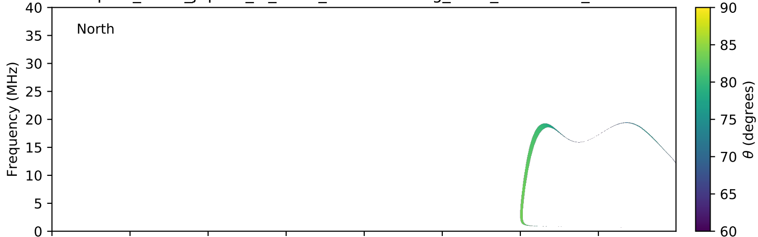
expres_earth_jupiter_io_isaac_lossc-wid1deg_3kev_20150208_v01.cdf
