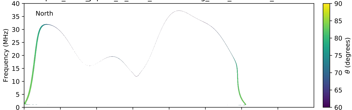
expres_earth_jupiter_io_isaac_lossc-wid1deg_3kev_20150207_v01.cdf
