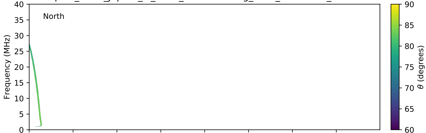
expres_earth_jupiter_io_isaac_lossc-wid1deg_3kev_20150206_v01.cdf
