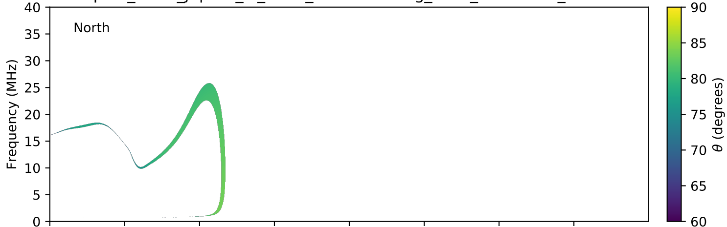
expres_earth_jupiter_io_isaac_lossc-wid1deg_3kev_20150204_v01.cdf
