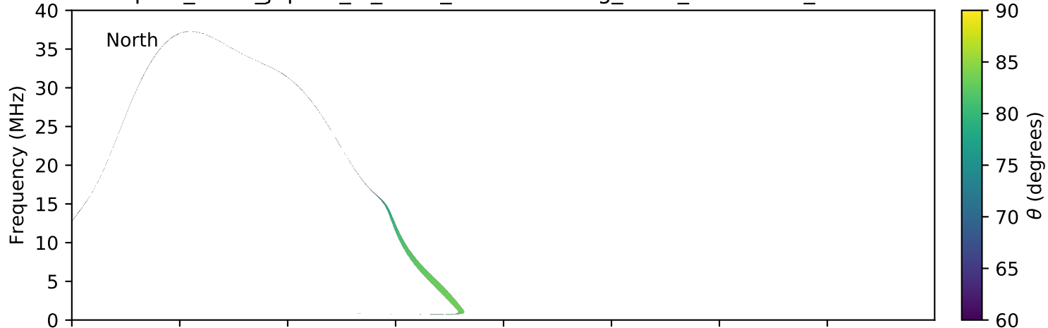
expres_earth_jupiter_io_isaac_lossc-wid1deg_3kev_20150202_v01.cdf
