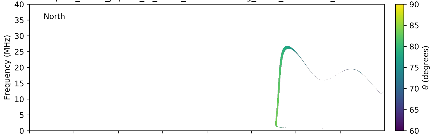
expres_earth_jupiter_io_isaac_lossc-wid1deg_3kev_20150201_v01.cdf
