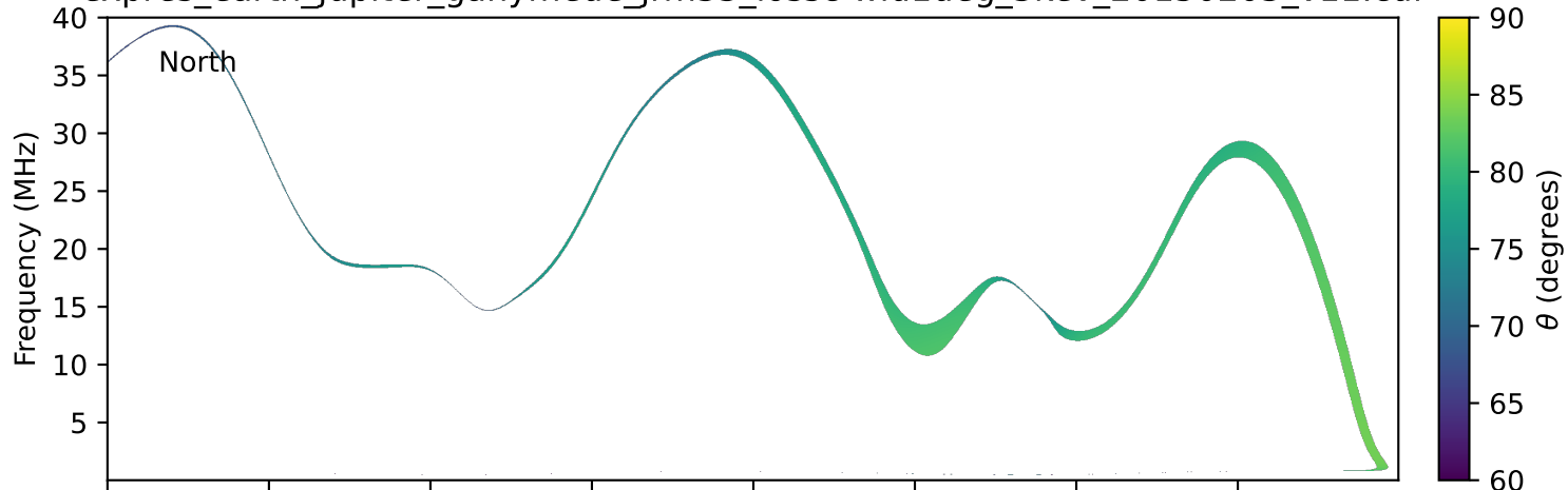
expres_earth_jupiter_ganymede_jrm33_lossc-wid1deg_3kev_20150203_v11.cdf
