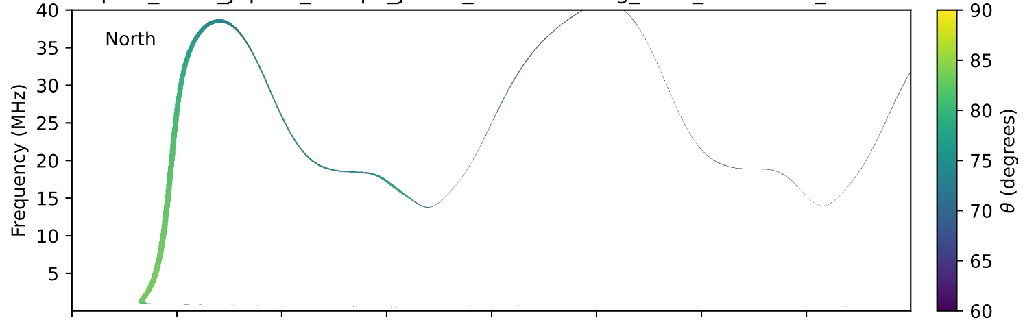
expres_earth_jupiter_europa_jrm33_lossc-wid1deg_3kev_20150228_v11.cdf
