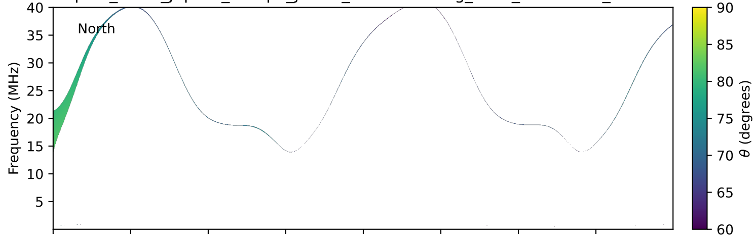
expres_earth_jupiter_europa_jrm33_lossc-wid1deg_3kev_20150214_v11.cdf
