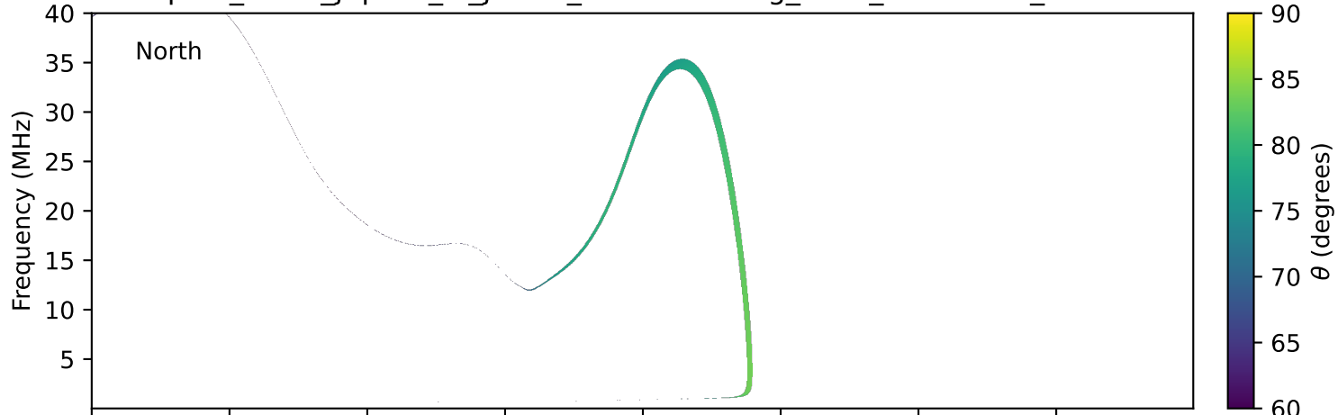
expres_earth_jupiter_io_jrm33_lossc-wid1deg_3kev_20140924_v11.cdf
