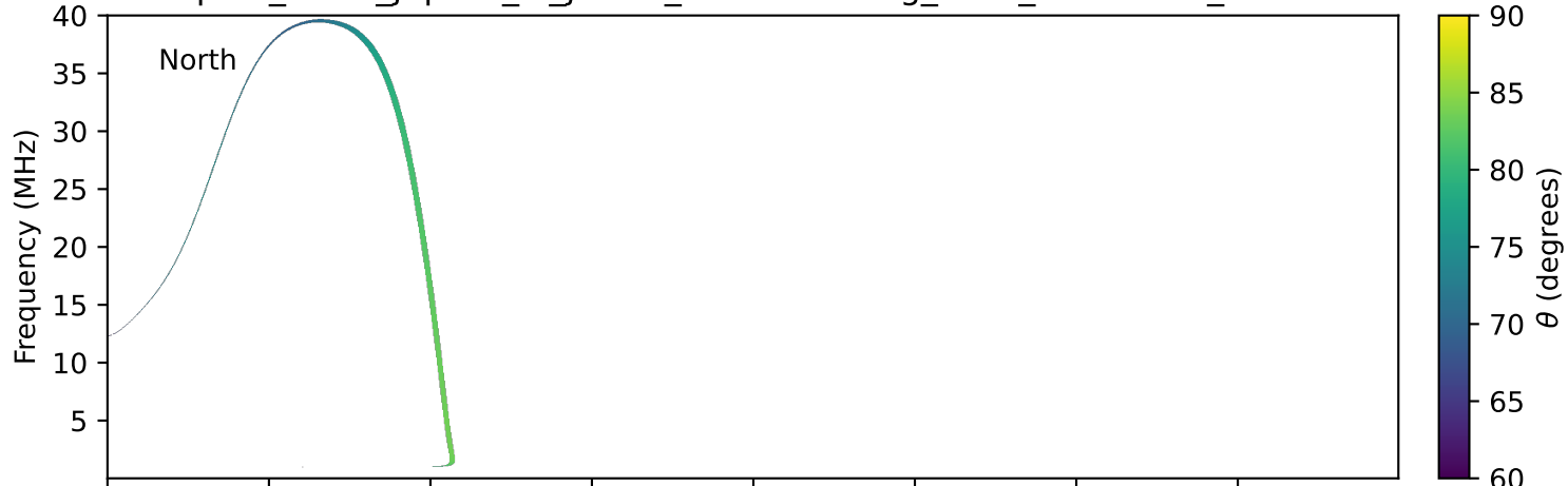
expres_earth_jupiter_io_jrm33_lossc-wid1deg_3kev_20140919_v11.cdf
