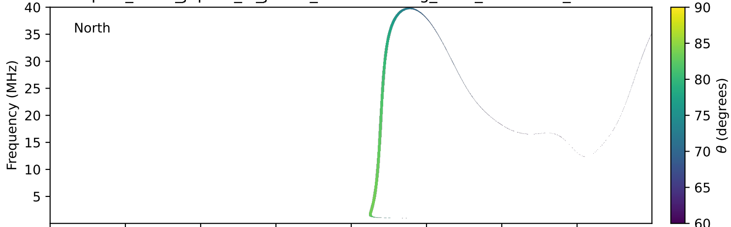
expres_earth_jupiter_io_jrm33_lossc-wid1deg_3kev_20140916_v11.cdf
