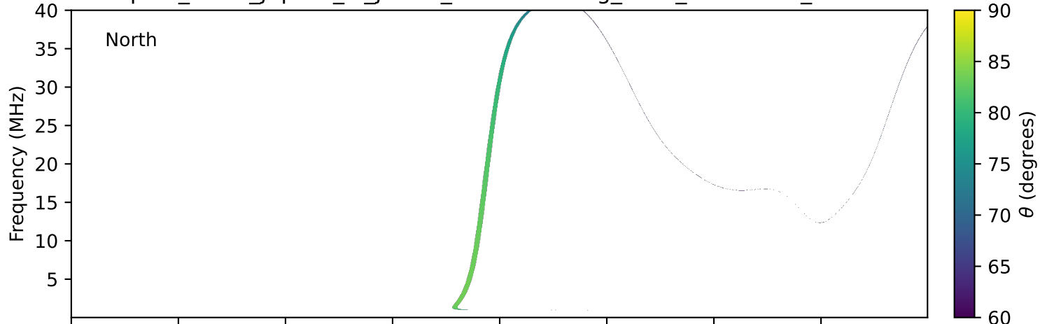
expres_earth_jupiter_io_jrm33_lossc-wid1deg_3kev_20140909_v11.cdf
