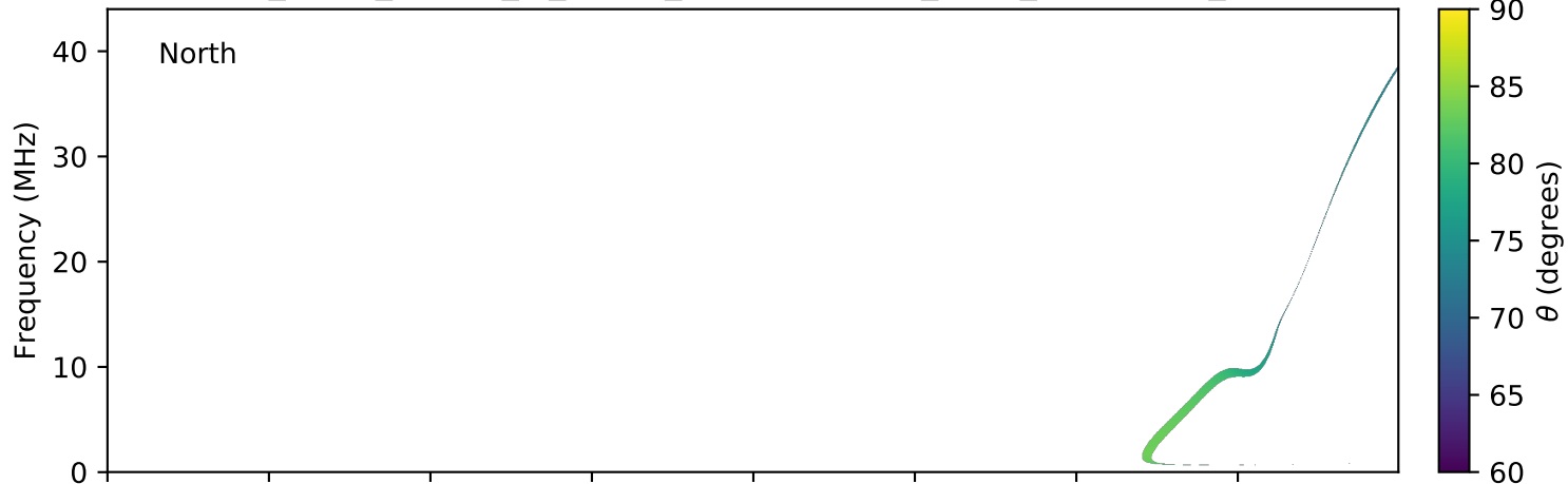
expres_earth_jupiter_io_jrm09_lossc-wid1deg_3kev_20140930_v01.cdf
