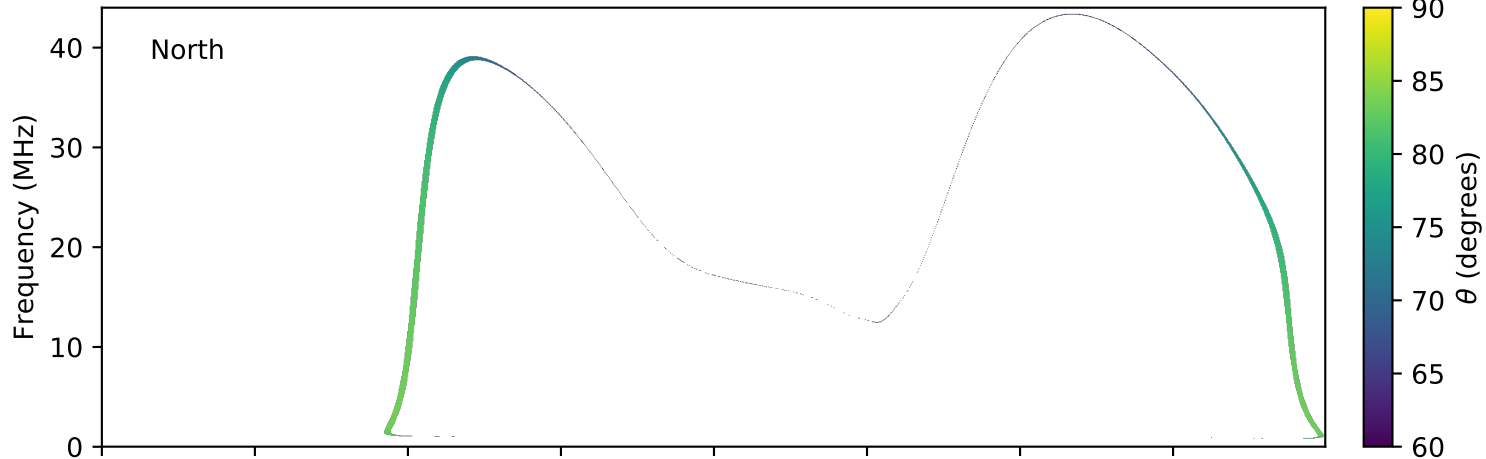
expres_earth_jupiter_io_jrm09_lossc-wid1deg_3kev_20140920_v01.cdf
