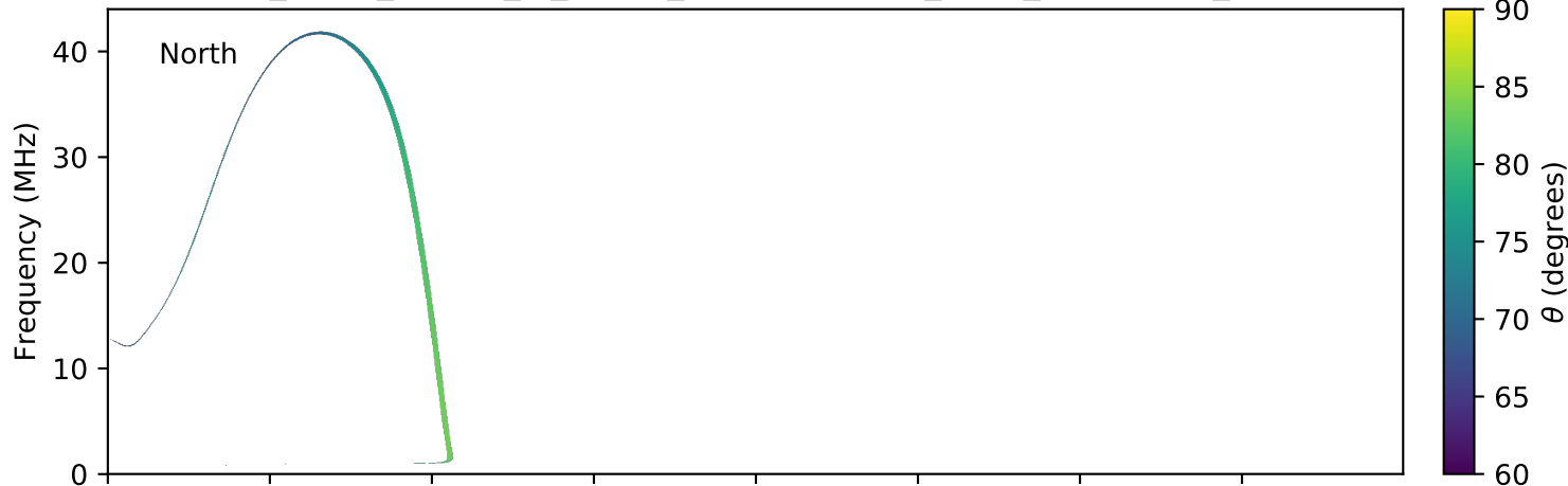
expres_earth_jupiter_io_jrm09_lossc-wid1deg_3kev_20140919_v01.cdf
