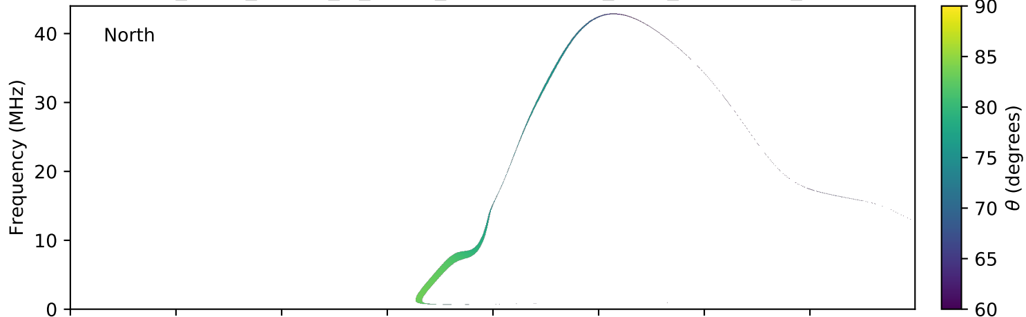
expres_earth_jupiter_io_jrm09_lossc-wid1deg_3kev_20140918_v01.cdf
