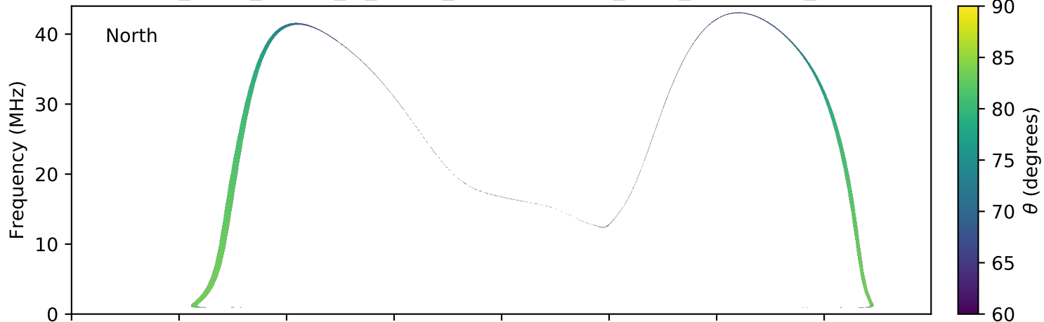
expres_earth_jupiter_io_jrm09_lossc-wid1deg_3kev_20140913_v01.cdf
