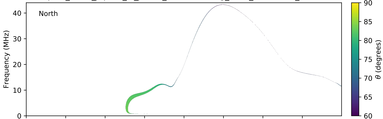
expres_earth_jupiter_io_jrm09_lossc-wid1deg_3kev_20140911_v01.cdf
