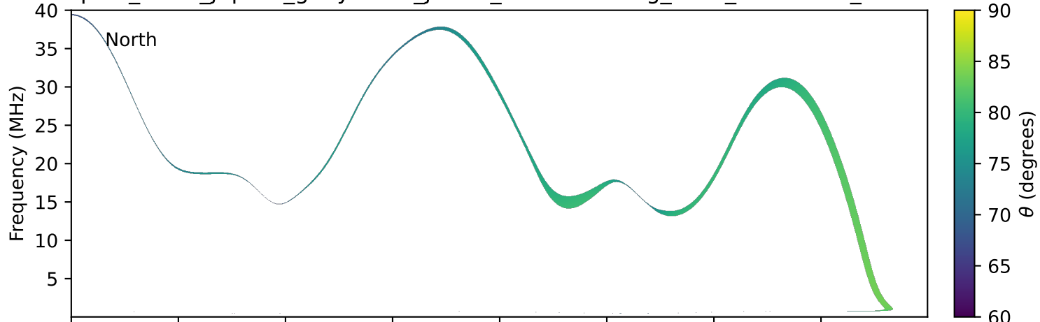
expres_earth_jupiter_ganymede_jrm33_lossc-wid1deg_3kev_20140920_v11.cdf
