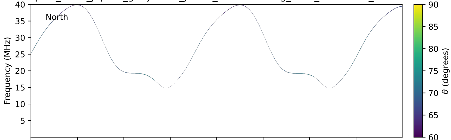
expres_earth_jupiter_ganymede_jrm33_lossc-wid1deg_3kev_20140919_v11.cdf
