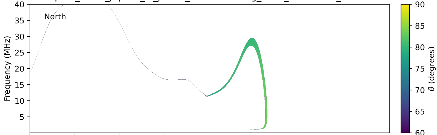
expres_earth_jupiter_io_jrm33_lossc-wid1deg_3kev_20140821_v11.cdf
