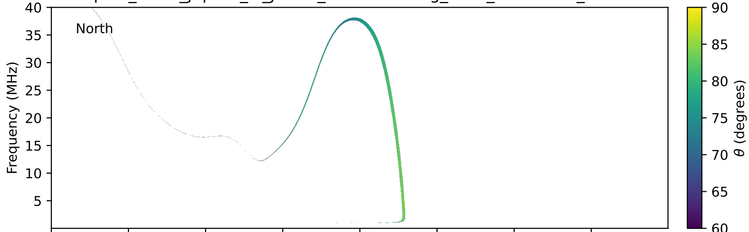
expres_earth_jupiter_io_jrm33_lossc-wid1deg_3kev_20140805_v11.cdf
