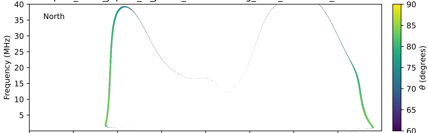
expres_earth_jupiter_io_jrm33_lossc-wid1deg_3kev_20140801_v11.cdf
