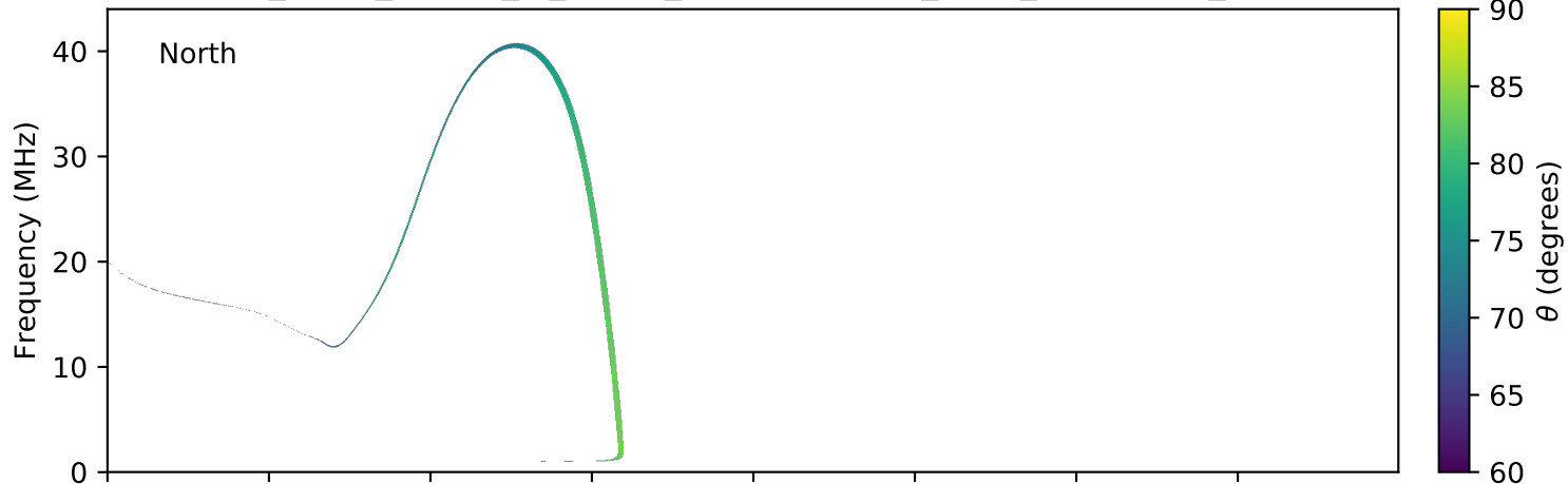
expres_earth_jupiter_io_jrm09_lossc-wid1deg_3kev_20140818_v01.cdf
