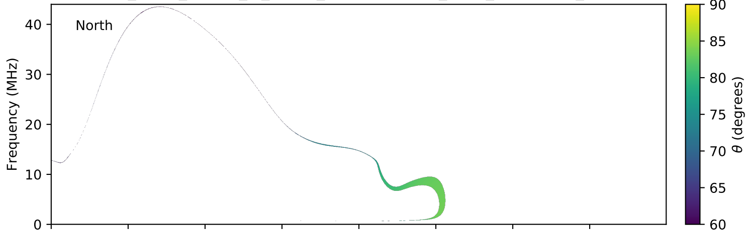
expres_earth_jupiter_io_jrm09_lossc-wid1deg_3kev_20140816_v01.cdf
