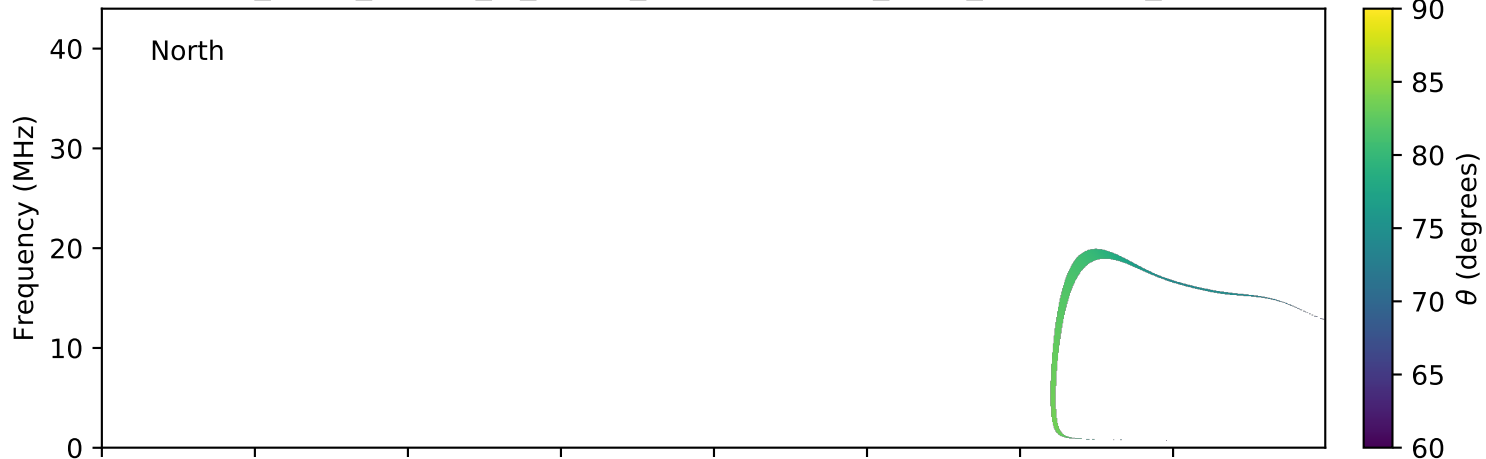
expres_earth_jupiter_io_jrm09_lossc-wid1deg_3kev_20140815_v01.cdf
