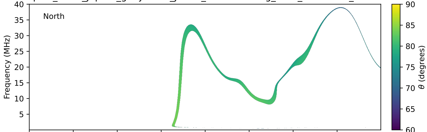
expres_earth_jupiter_ganymede_jrm33_lossc-wid1deg_3kev_20140831_v11.cdf
