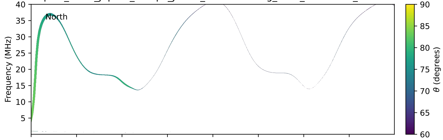
expres_earth_jupiter_europa_jrm33_lossc-wid1deg_3kev_20140819_v11.cdf
