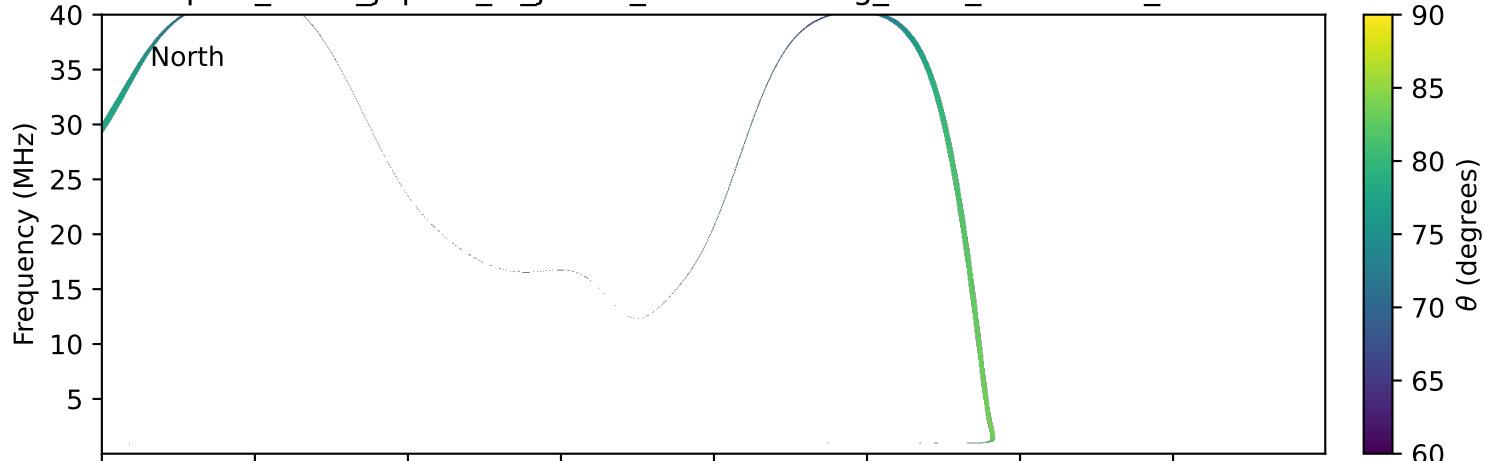
expres_earth_jupiter_io_jrm33_lossc-wid1deg_3kev_20140627_v11.cdf
