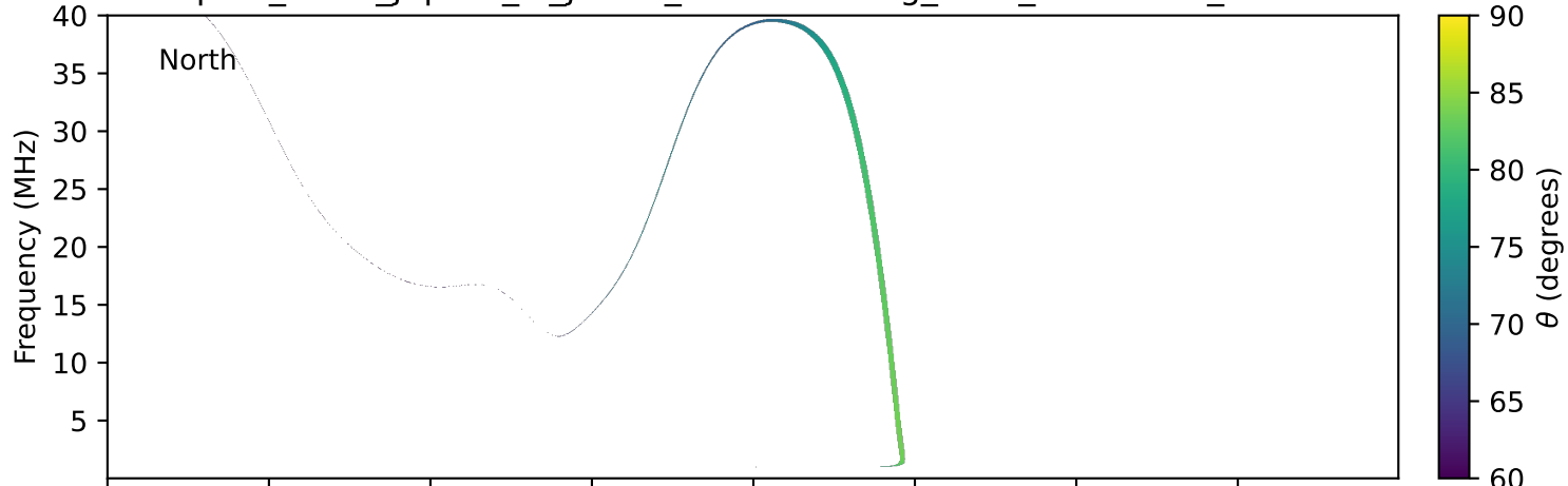
expres_earth_jupiter_io_jrm33_lossc-wid1deg_3kev_20140606_v11.cdf
